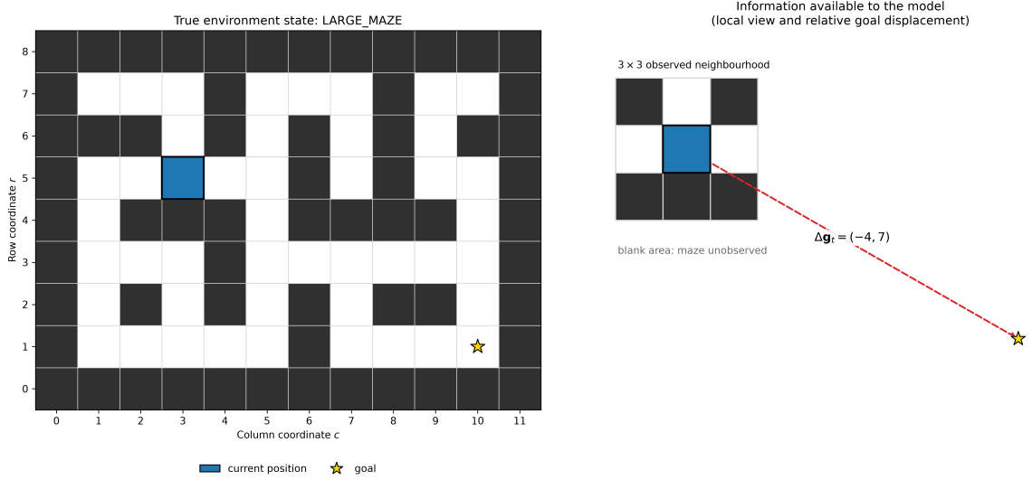
Figure 3: Comparison of the true maze state and the corresponding partial observation at the same time step. The left panel shows the full LARGE_MAZE layout, the agent’s current position, and the goal using absolute grid coordinates. The right panel shows only the local 3 \times 3 neighbourhood and the goal’s relative displacement.
